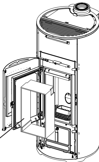
UNPACKING HALO CLADDING
