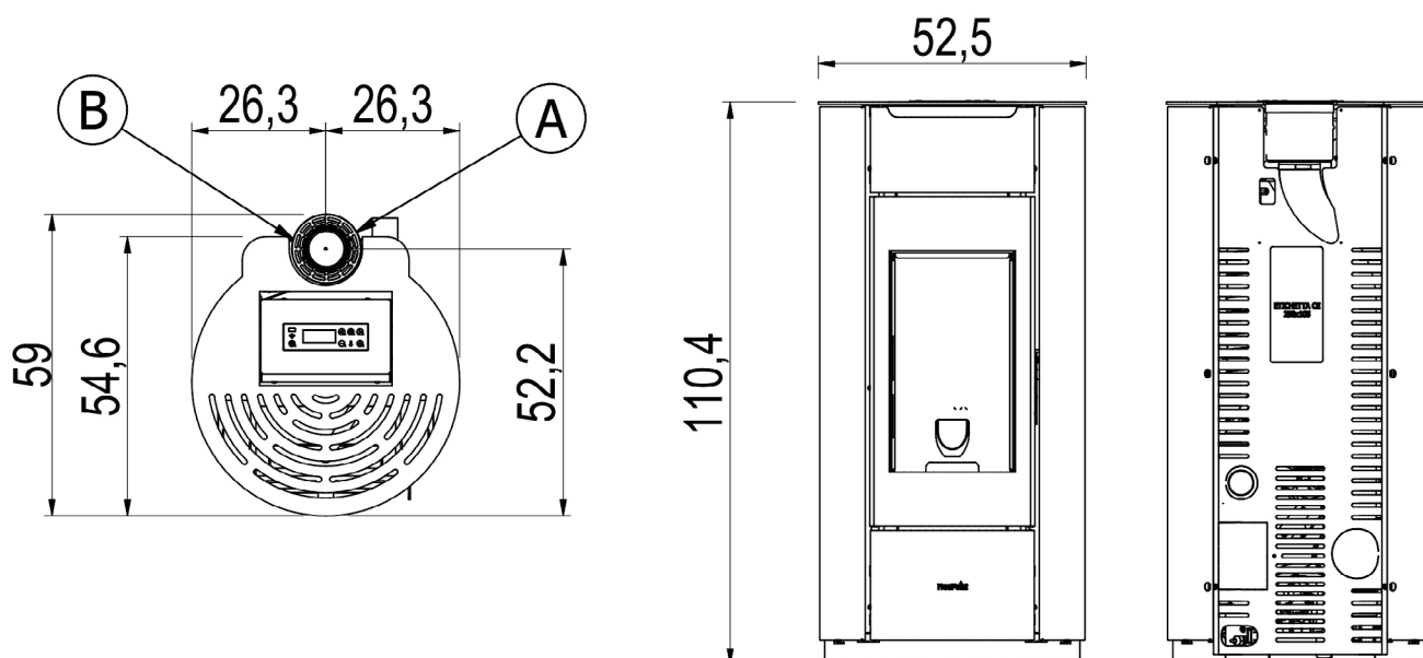
Fig. 18 - EOS 8 BI-FLUX K1 - EOS 8 BI-FLUX T1 - EOS 6 BI-FLUX T1
