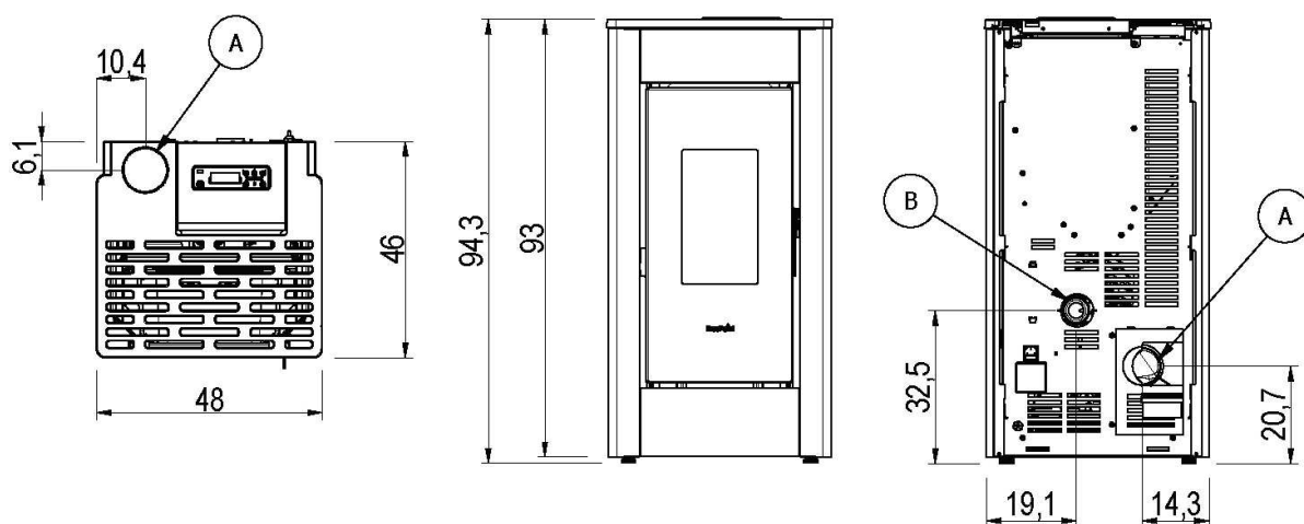
Fig. 17 - Dimensiones generales: ---
