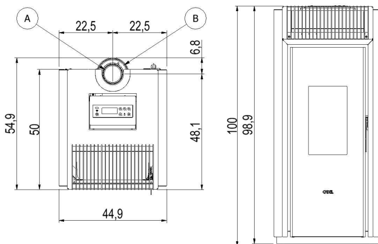
Fig. 24 - BOLD 7 UP TWIN
