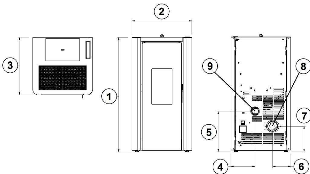
Fig. 26 - Dimensiones generales: ---
