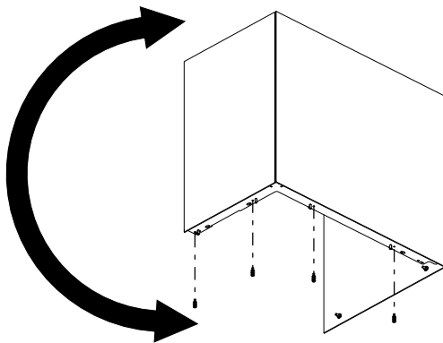
Fig. 20: Prepare steel cladding
