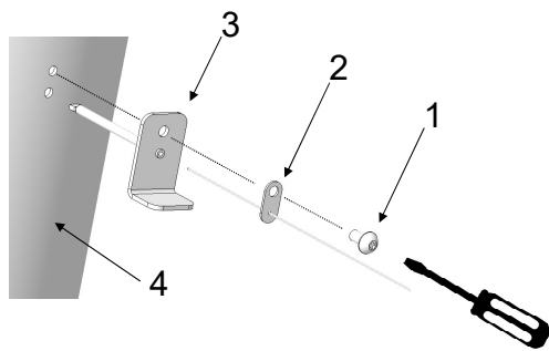
Fig. 6: Mounting the temperature sensor
