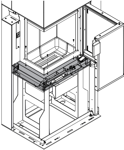
Fig. 26: Remove the trim at the bottom
