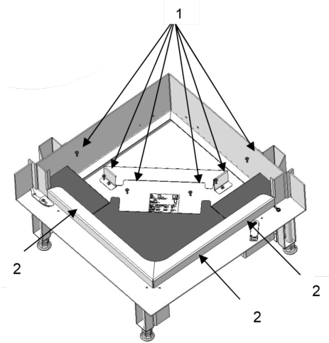
Fig. 9: Removing 55x parts
