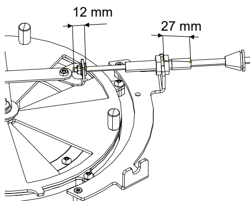
Fig. 14: Raccorder le câble Bowden
