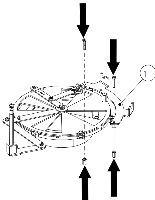
Fig. 11: Installing the installation kit
