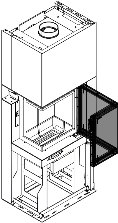
Fig. 24: Opening door
