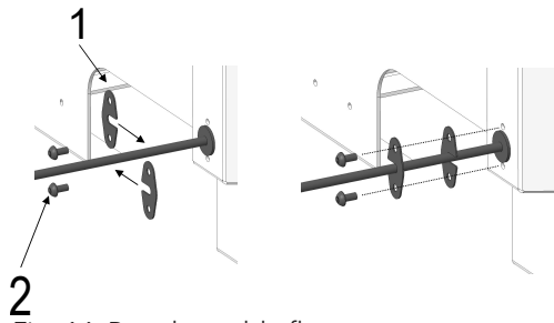
Fig. 16: Bowden cable flange
