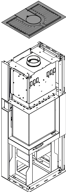
Fig. 19: Remove cover
