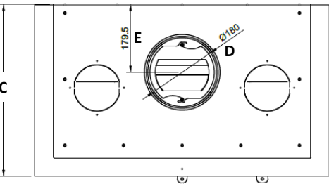
Upper view
