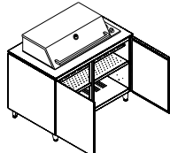
48 Drop-in grill 1200 x 770 x 915mm 48" x 30" x 36"
