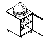
24 Charcoal grill 600 x 770 x 915mm 24" x 30" x 36"
